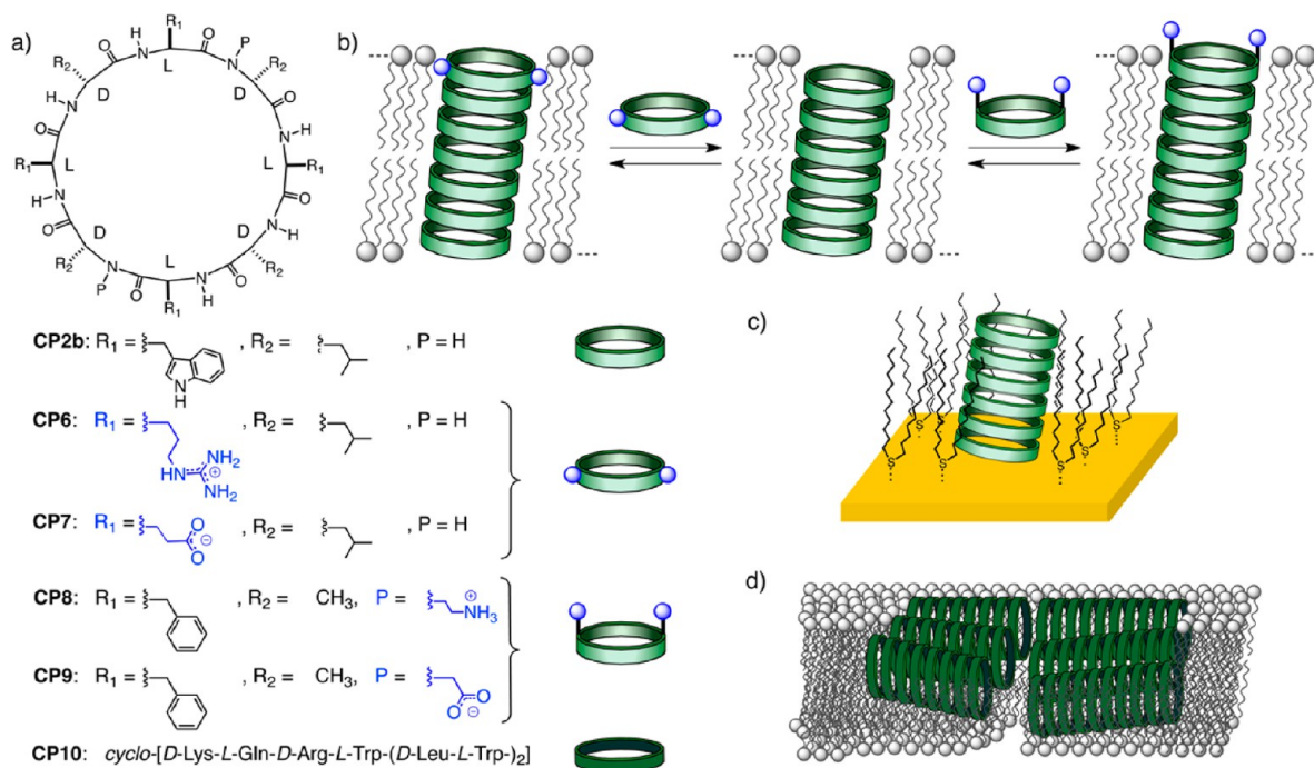
FIGURE 4. (a) Structures of CP2b, CP6–10. (b) Mode of interaction of the CP caps (CP6–9) with the transporting ensemble of CP2b to afford heteromeric transmembrane channels. (c) SCPN2b embedded in the gold SAMs for the construction of selective ion sensors. (d) Proposed model of parallel nanotube orientation for amphiphilic antibacterial D,L - \alpha -cyclic peptides (CP10).
