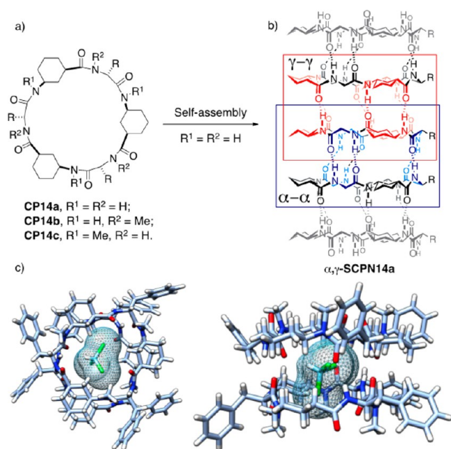
FIGURE 6. (a) Structure of \alpha,\gamma -CPs CP14a-c. (b) Different hydrogen-bonding pattern in the tubular arrangement of \alpha,\gamma -SCP. (c) Crystal structure of dimeric assembly of CP14c (R=Bn), in which one chloroform molecule occupies their cavity: (left) top view; (right) side view.
