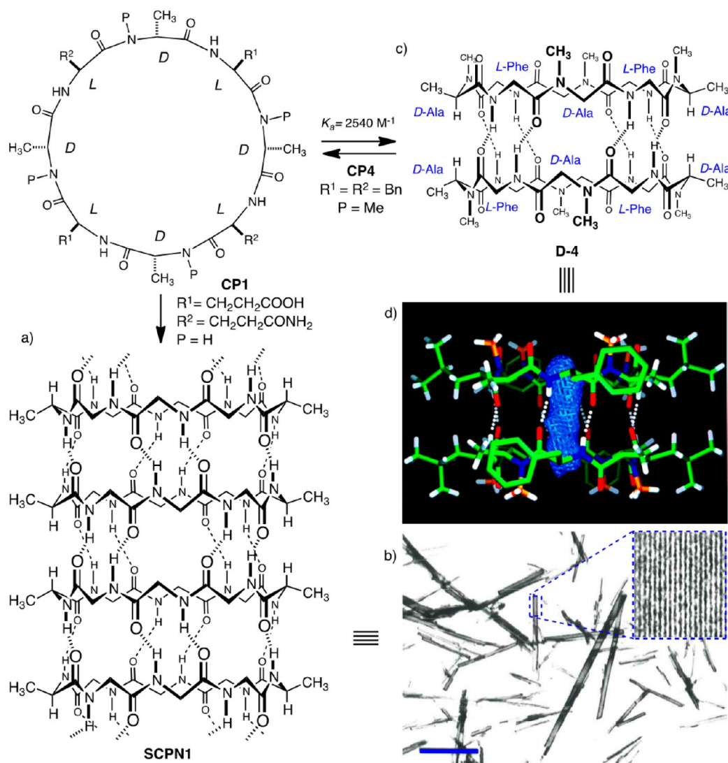
FIGURE 1. CP1 and CP4. (a) Self-assembled nanotube structure of CP1 (most of the side chains are omitted for clarity). (b) Electron microscopy low-magnification image of nanotube suspension adsorbed on a carbon support film (scale bar 1 \mu\text{m} ); inset shows low-dose image enhancement of a single crystal and reveals the longitudinal striations that correspond to each nanotube. (c) Cylindrical dimer of CP4. (d) Crystal structure of D4 emphasizing the internalized water binding sites (blue rod).
