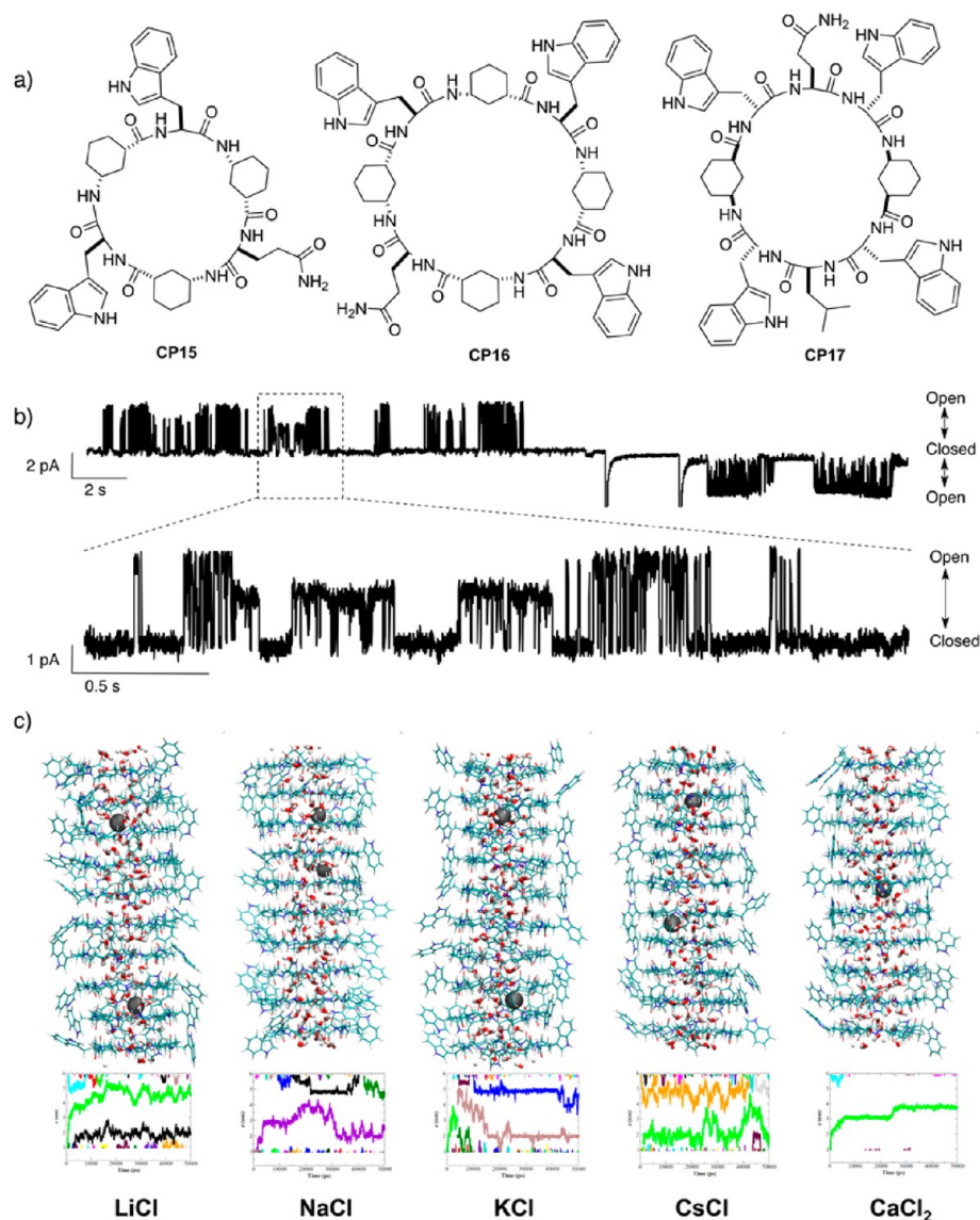
FIGURE 7. (a) Structure of \alpha,\gamma -CPs CP15–17. (b) Single-channel recordings of \text{Na}^+ current through CP16 channels (+100 and -100 mV) and 3.0 s detail of the trace showing two different current levels (1.8 and 3.1 pA). (c) Snapshots of simulated SCPNs in 0.5 M electrolyte solutions after 25 ns of simulation (lipids and external water and ions have been removed for clarity) and Z coordinate for the ions inside the nanotube along the trajectory. 38 Part of this figure is reproduced by permission of The Royal Society of Chemistry.
