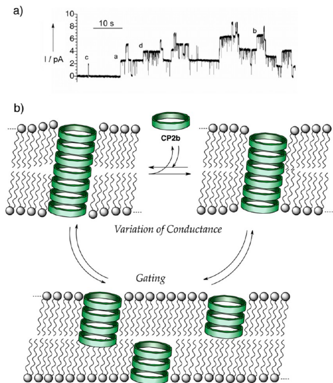
FIGURE 3. (a) Different conducting states recorded at +100 mV, showing at least four working channels formed by CP2b in L\text{-}\alpha -lecithin bilayers in 1 M KCl. (b) Probable mechanisms of gating and of variable conductance events.
