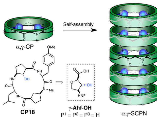
FIGURE 8. Structure of CP18 and model for nanotube formation showing the hydroxyl groups (blue color) projected toward the cavity.
